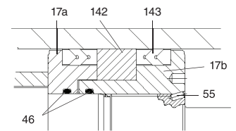
Chevron Piston
