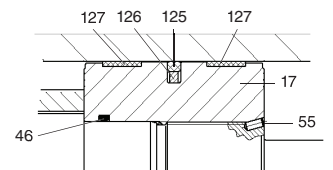
Standard Piston
